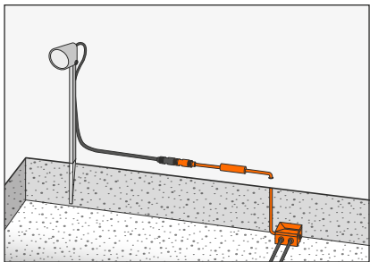
Erd-Anschluss-Kit underground connection kit
