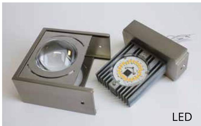
Focus 100 LED
